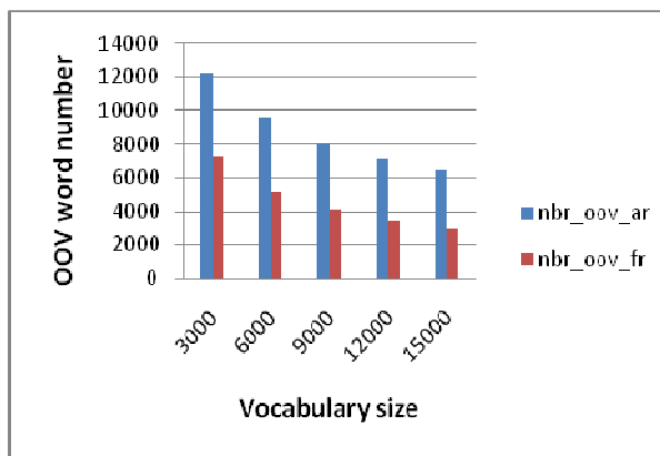
Figure 3: variation in the number of words oov depending on the size of the training vocabulary.
