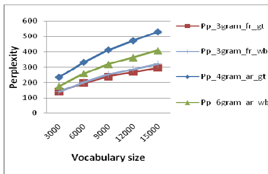
Figure 2: evolution of perplexity of Arabic (ar) and French (fr) n-gram models depending on the size of the vocabulary.
