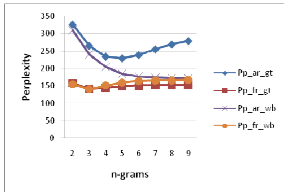
Figure 1: comparison of perplexities obtained for Arabic (ar) and French (fr) n-gram language models with Good Turing (gt) and Witten Bell (wb) smoothing techniques.
