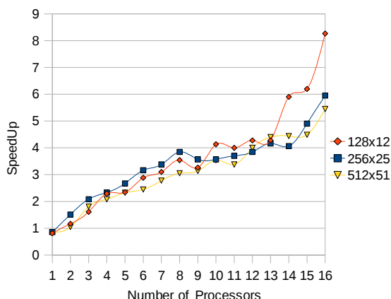
Figure 7: Speedup using a mass-spring mesh simulation by domain decomposition. The sequential time for each case is : 125ms (128x128), 500ms (256x256), 2.2s (512x512)
