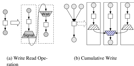
Figure 3: Control tasks employed to guarantee data access coherence between different partitions. On a write/read operation the reader waits for the data to be produced by the writer. In a cumulative write operation all the writes are performed in a temporary buffer that will be further accumulated by the Reducer.
