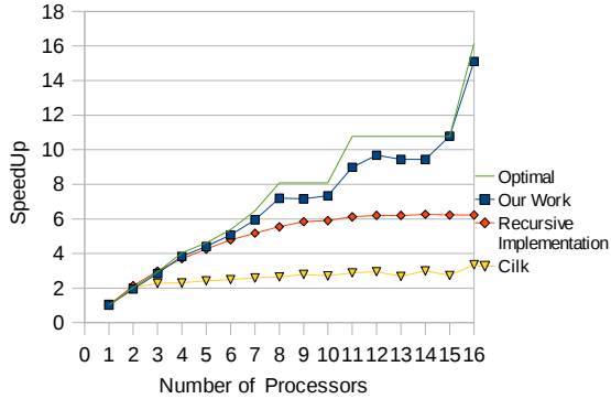
Figure 5: Speedup using 64 identical bars of size 16x4x4 without collision. T_1 = 150ms
