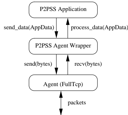
Figure 1: Simulator architecture.
