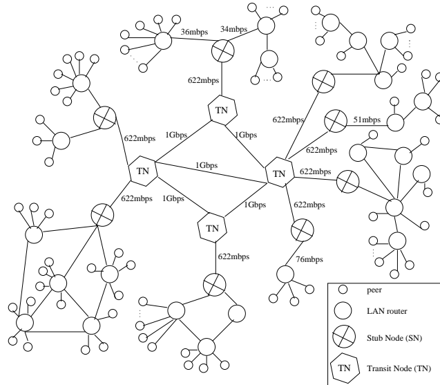
Figure 2: Three-level hierarchical random graph of Experiment 1.
