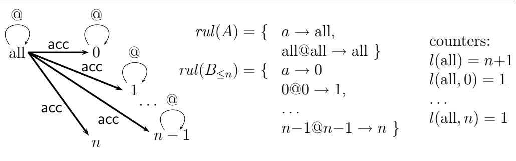
Figure 6: Rule (frb_{/2}) can infer, for all 0 \leq i \neq j \leq n , the clause frb(all, i) :- acc(all, j) .
