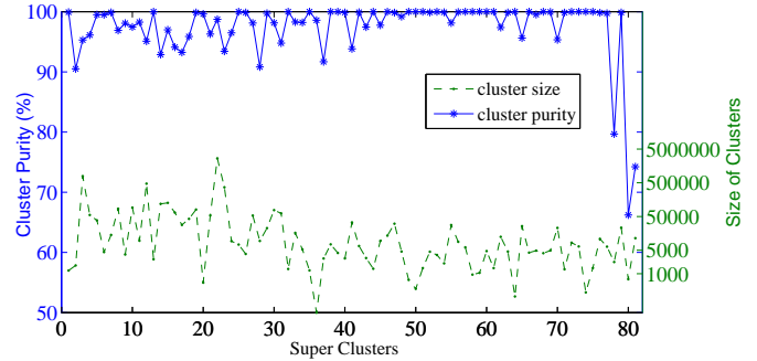
Fig. 10. Offline Monitoring: Purity of Super Clusters
