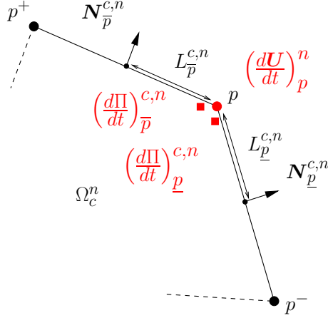
Figure 11: Localization of the time derivatives of the nodal pressures and velocity at point p viewed from cell \Omega_c^n .
