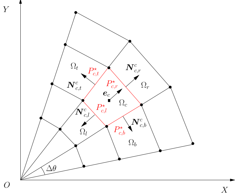
Figure 3: Equal angle polar grid.
