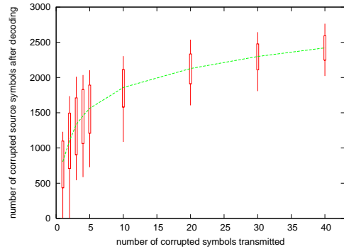
Fig. 1. Number of corrupted source symbols after decoding (average/min/max/90 % confidence interval) W.R.T. the number of corrupted symbols received.
