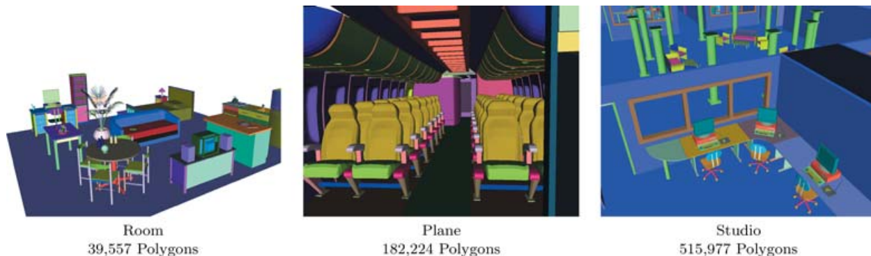
Fig. 7. Scenes used for testing the object congruency descriptor. In each scene, the descriptor has been used to detect objects with similar geometry (but possibly different meshes) up to a rigid transform. Objects found to be congruent are displayed with the same color.
