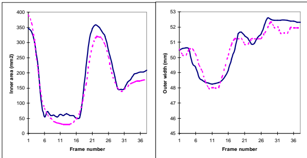
Figure 4. Left : Inner contour area ( \text{mm}^2 ); Right : Outer contour width (mm); measured parameter is in dot line, predicted in full line.
