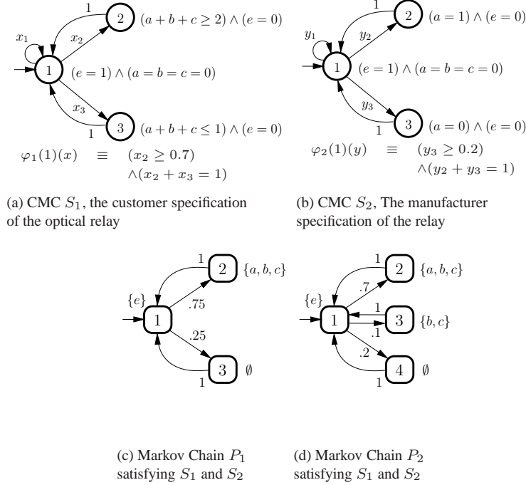
Figure 2: Two specifications (CMCs) and two implementations (MCs) of an optical relay
