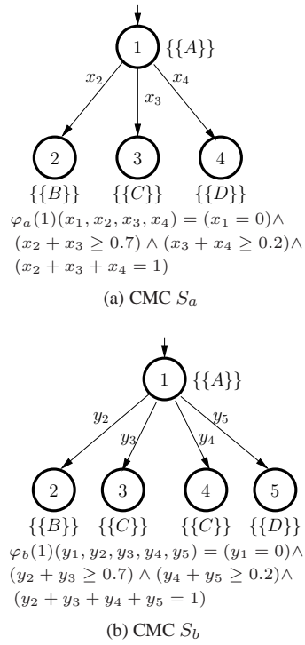
Figure 8: CMCs S_a and S_b
