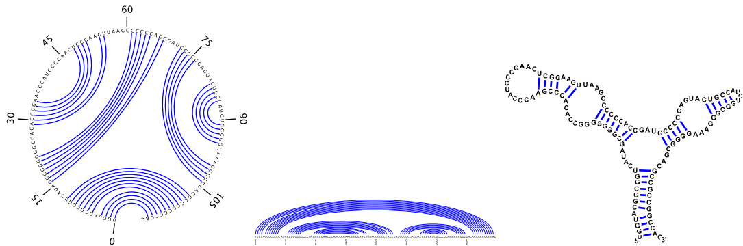
Figure 1: Depiction of 5S ribosomal RNA from M. Jannaschii with GenBank accession number NC_000909. Equivalent representations as ( Left ) outerplanar graph (also called Feynman circular diagram), ( Middle ) Feynman linear diagram, ( Right ) classical diagram (most familiar to biologists). The sequence and secondary structure were taken from the 5S Ribosomal RNA Database [20], and the graph was created using jViz [21].
