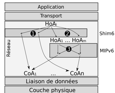
Figure 1. Architecture de la pile MipShim6
