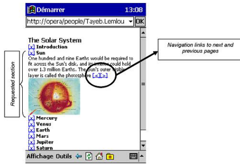
Fig. 3. Content pagination and links generation
