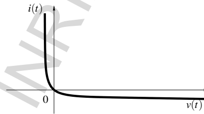
Fig. 1.1c. The graph of the Shockley's law
