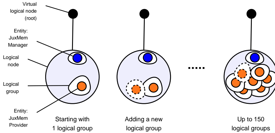
FIG. 4 – Expanding the JUXMEM topology by sequentially adding new providers into the same cluster group.
