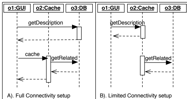
Figure 3. Sequence diagrams for full and low connectivity configurations.
