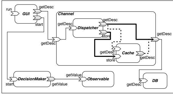
Figure 10. FraSCAti example with limited and full connectivity.
