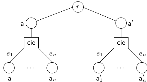
Fig. 5.5 A p-document of \text{PrXML}_{|\mathcal{W}}^{\{\text{cie}\}} that can be neither efficiently v-translated nor o-translated to \text{PrXML}_{|\mathcal{W}}^{\{\text{ind,mux,exp}\}}
