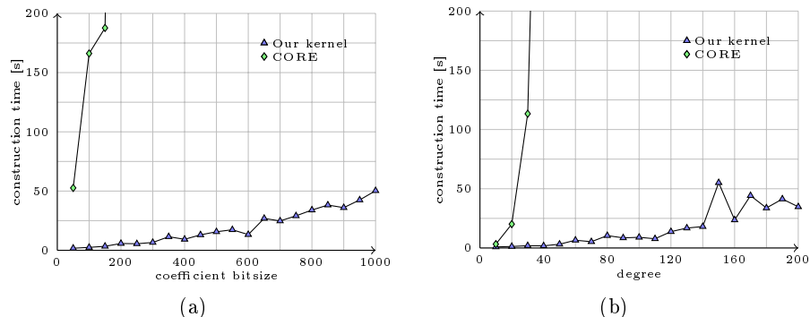
Fig. 5. Arrangements of five polynomials, shifted four times each, (a) of degree 20 and varying bitrate and (b) of bitrate 32 and varying degree.
