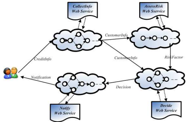
Fig. 2. Decentralized Credit Approval process
