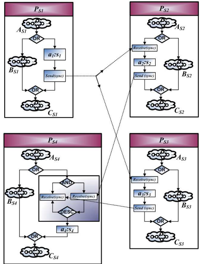
Fig. 8. Decentralized discriminator pattern
