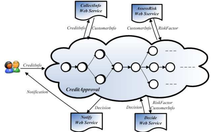
Fig. 1. Centralized Credit Approval process
