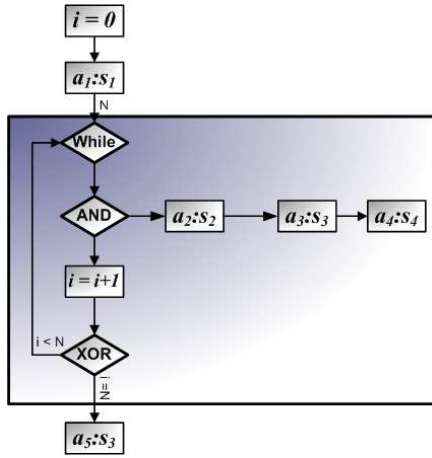
Fig. 5. Multiple instances pattern
