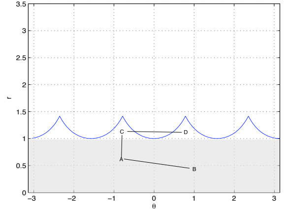
Fig. 4. Image plane in r-\theta space.
