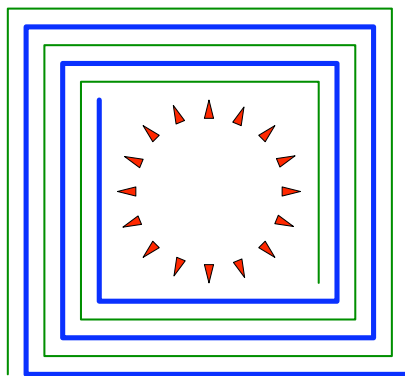
Figure 3: Curves and obstacles that admit \Omega(mnk^2) minimal relative homotopy classes and \Omega(mnk^4) relative homotopy classes of direct geodesics.
