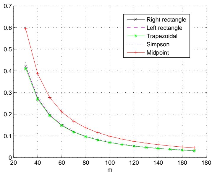
Figure 4: M_m^+(0, 0, T)
