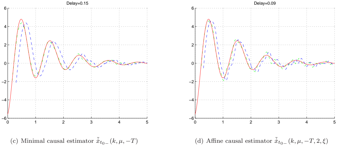
Figure 8: Time-delayed estimations and delay-free estimations with a moving window of length T = 60T_s = 0.3
