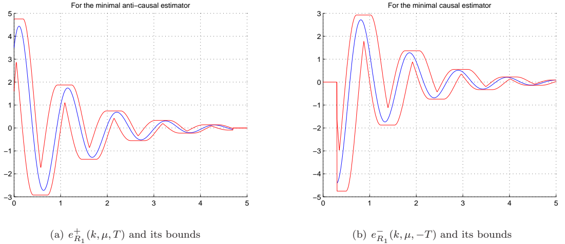
Figure 1: Comparisons between the bias term errors for the minimal estimators and their bounds
