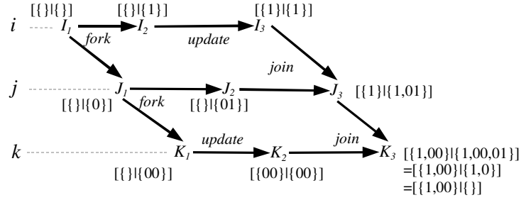
Fig. 13. Example of the use of version timestamps (VTs). An object starts as a single replica I_1 with a VT of \{\{\}\}|\{\} . It is forked into two replicas I_2 and J_1 . Site i updates the replica, which becomes I_3 . Merging replicas I_3 and J_2 detects no conflict, as I_3 dominates J_2 , as apparent from the fact that \{1\} \supset \{\} . In contrast, concurrent updates are detected when merging replicas J_3 and K_2 , as neither of the upd-ids \{00\} and \{1\} subsumes the other.
