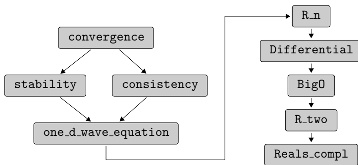
Figure 4: Dependency graph of the Coq development. On the left are the files from the convergence proof. The other files correspond to the reusable library.
