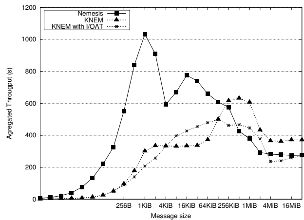
Figure 4. Aggregated throughput during a IMB Scatter with 16 processes on Idkonn24.
