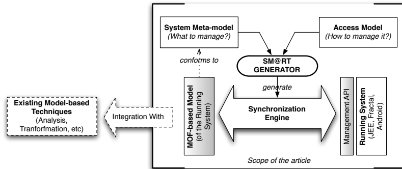
Fig. 2. Generation of Synchronization Engine: Approach Overview
