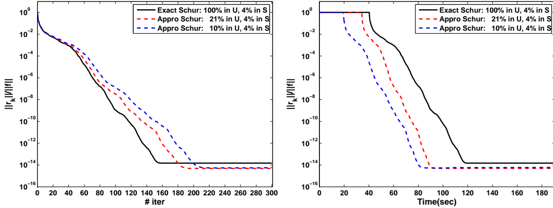
(a) Heterogeneous diffusion Problem 1 with Convection 1 (history v.s. iterations).
