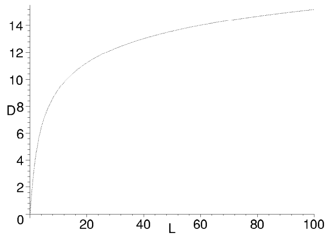
(b) A distance D assuring a lack of interferences according to the radius L of the network with \alpha = 2 , R = 1 and Q = 10 .
