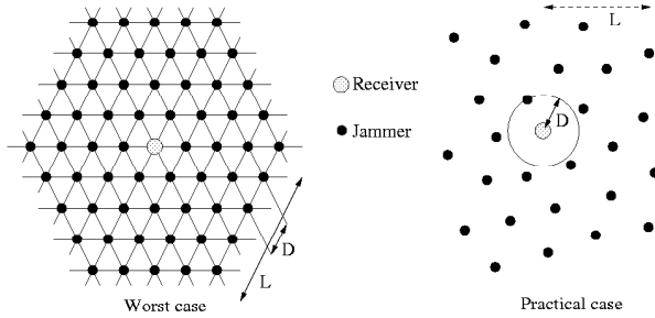
Fig. 1. Two situations where the transmitters are within a distance D from each other, with L the distance of the jammer the furthest in the network. On the left, “a worst case”, on the right “a practical situation”.
