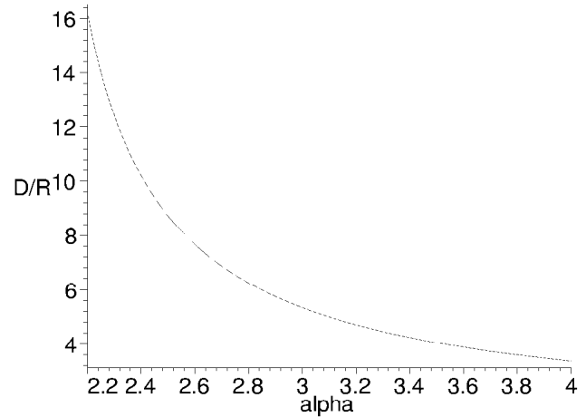
(a) A ratio D/R assuring a lack of interferences according to the attenuation coefficient of power \alpha with Q = 10 .
