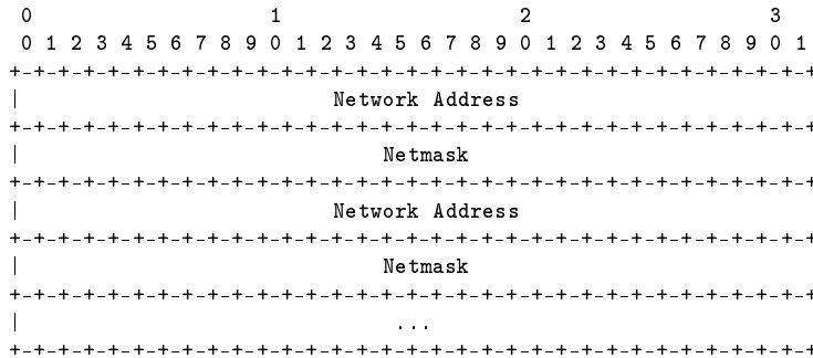
Figure 5: Layout of OLSR HNA messages
