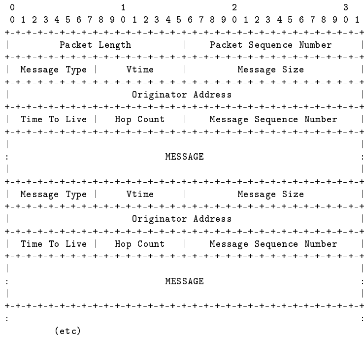
Figure 1: Layout of OLSR general packet format
