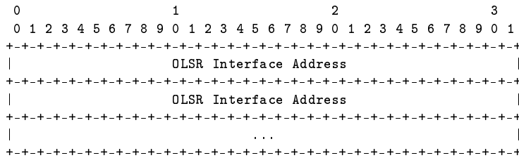
Figure 2: Layout of OLSR MID messages
