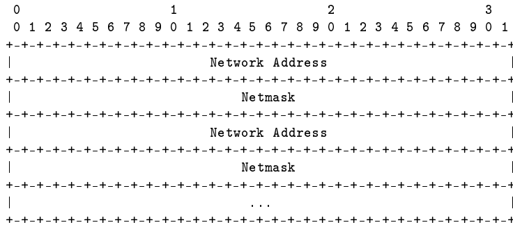
Figure 5: Layout of OLSR HNA messages
