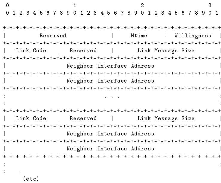
Figure 3: Layout of OLSR HELLO messages
