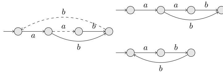
Figure 1: A modal specification MTS and some associated models
