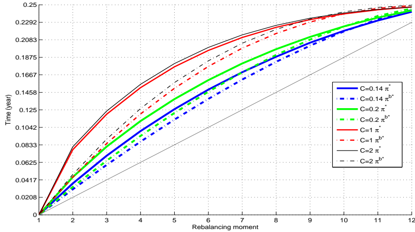
Figure 2: Parametric and non parametric optimal rebalancing grids for different choices of parameter C with N = 12 and K = 99 (Digital option).
