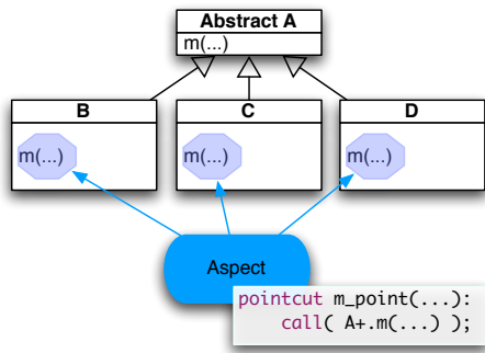
Fig. 1. Aspect applied to three different classes
