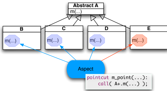
Fig. 2. Aspect applied to a class that does not need it
