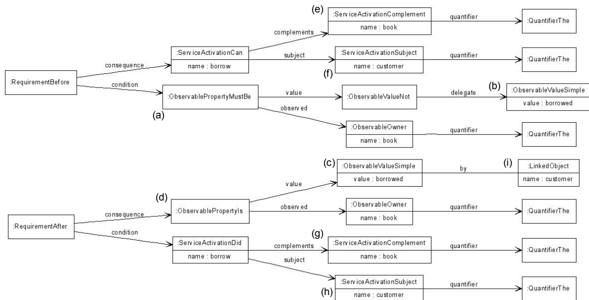
Figure 4 – A RDM model corresponding to the requirements (1) and (2) of the Figure 1
