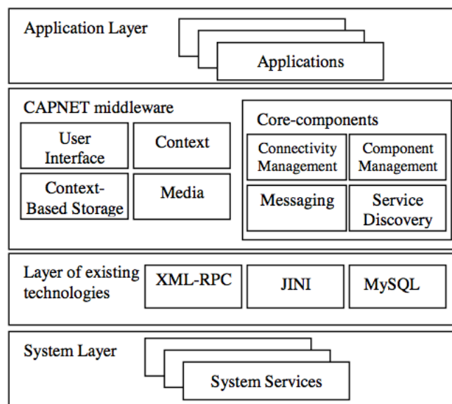
Fig. 8. CAPNET Architecture
