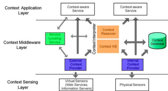
Fig. 7. SOCAM Architecture
