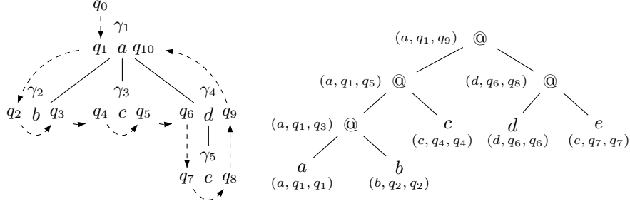
(a) A run of the NWA A on t \in \mathcal{T}_\Sigma . (b) A run of the corresponding nTA A' on curry(t) .
