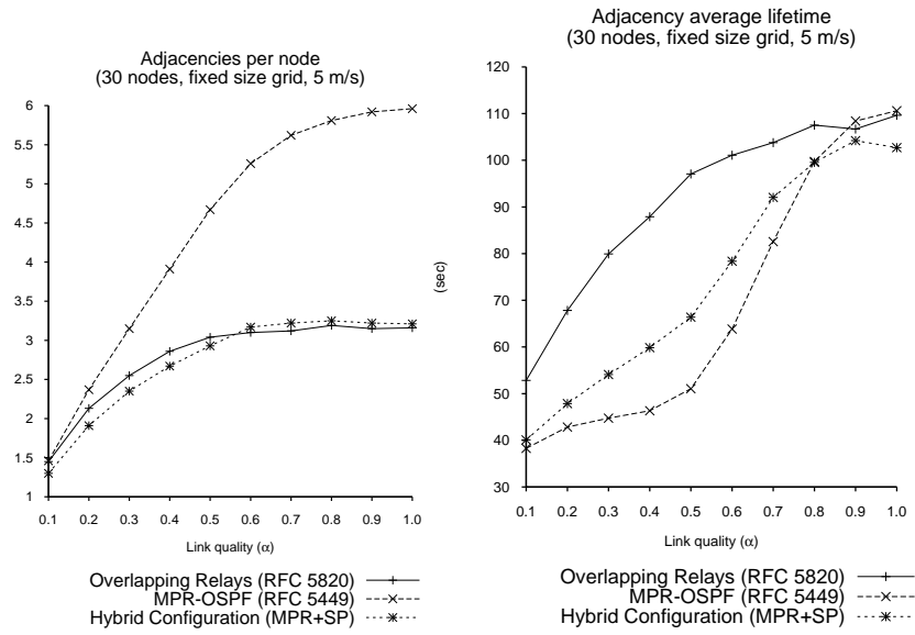
Figure 13: (a) Average number of adjacencies per node and (b) average adjacency lifetime (30 nodes, fixed size grid, 5 m/s).
