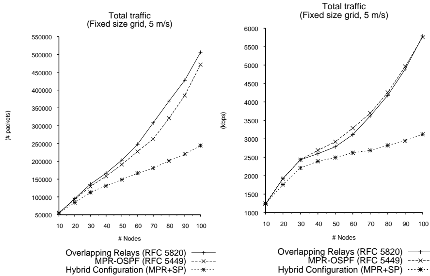
Figure 16: Total traffic in (a) number of packets and (b) Kbps (fixed size grid, 5 m/s).
