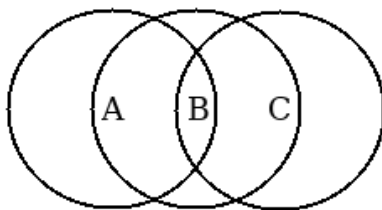
Figure 2: Non-transitivity issues: the hidden node problem. B can hear both A and C on the same interface, but A and C do not hear each other on this link.
