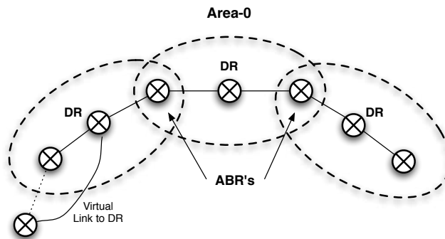
Figure 1: An OSPF autonomous system splitted in different areas (Area-0 is the backbone area).
