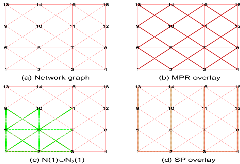
Figure 7: Example of static network and the components of the topology subgraph reconstructed by node (1): (a) Network graph, (b) Path MPR overlay, (c) 1-hop and 2-hop neighborhood of (1), and (d) (a possible) Smart Peering overlay.
