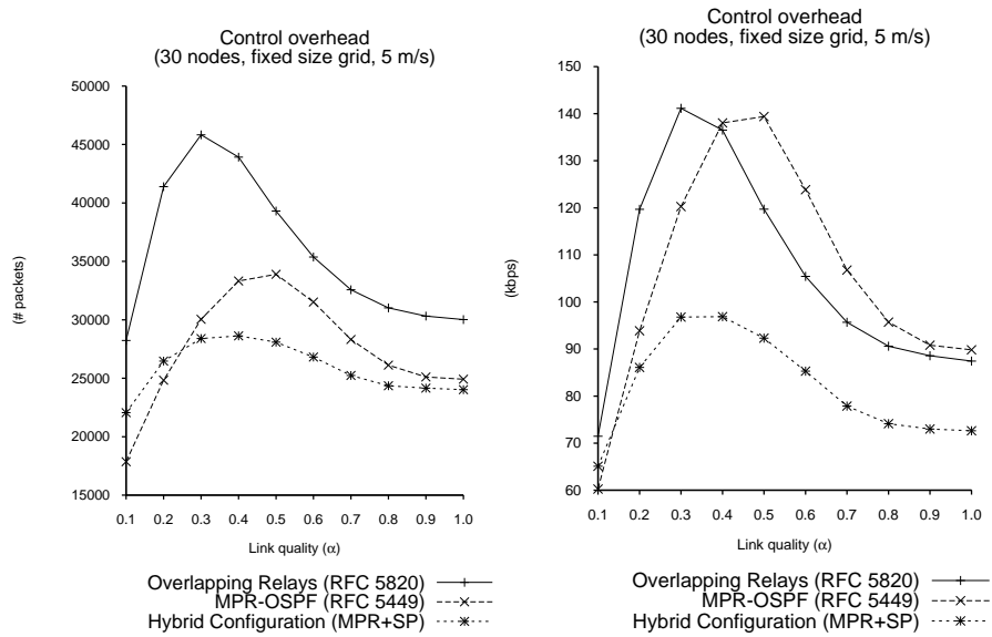
Figure 17: Control traffic overhead (a) number of packets and (b) Kbps (30 nodes, fixed size grid, 5 m/s).
