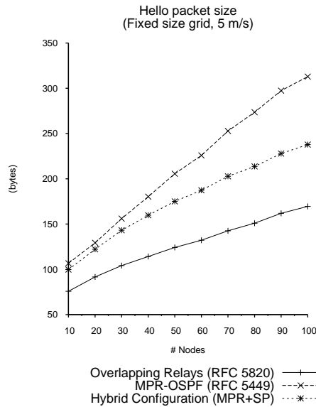
Figure 12: Average size of Hello packets (fixed grid, 5 m/s).
