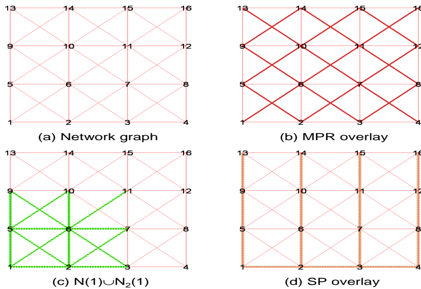
Figure 7: Example of static network and the components of the topology subgraph reconstructed by node (1): (a) Network graph, (b) Path MPR overlay, (c) 1-hop and 2-hop neighborhood of (1), and (d) (a possible) Smart Peering overlay.
