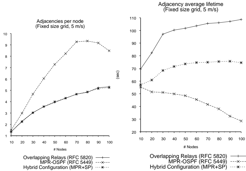
Figure 11: (a) Average number of adjacencies per node and (b) average adjacency lifetime (fixed size grid, 5 m/s).
