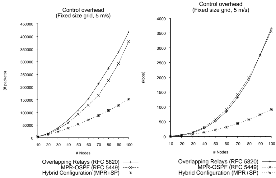
Figure 15: Control traffic overhead in (a) number of packets and (b) Kbps (fixed size grid, 5 m/s).
