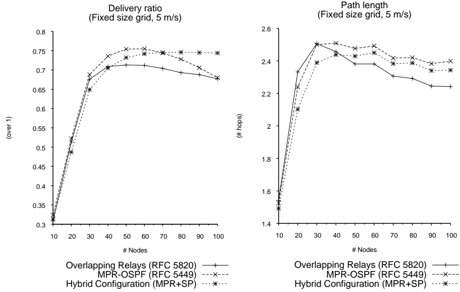
Figure 9: (a) Delivery ratio and (b) path length (fixed size grid, 5 m/s).
