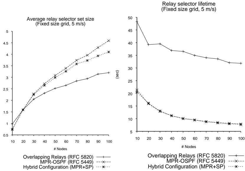
Figure 10: (a) Average number of relays per node and (b) average relay lifetime (fixed size grid, 5 m/s).
