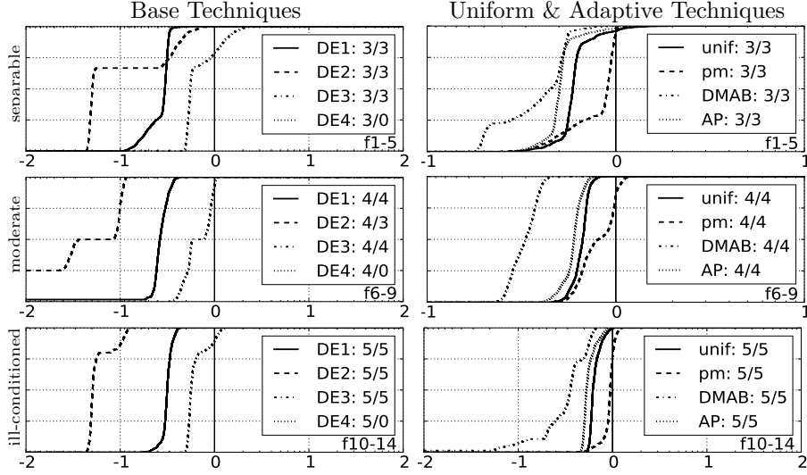
Fig. 2. Empirical cumulative distribution function of the speed-up ratios in dimension d = 20 for the F -AUC-Bandit compared with the base techniques (left) and with the uniform and adaptive ones (right). The speed-up ratios are the pairwise ratios of the number of function evaluations for F -AUC-Bandit to surpass the target function value 10^{-8} over the one of the baseline techniques over all trials of one functions. Pairs where both trials failed are disregarded, pairs where one trial failed are visible in the limits being > 0 or < 1 (for this reason, the lines for DE4 are not visible, as they coincide with the axes). The legends also indicate the number of functions that were solved in at least one trial ( F -AUC-Bandit first).
