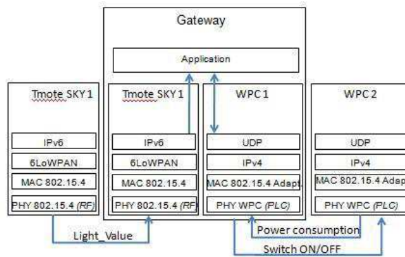
Figure 10: Communication layers
