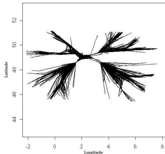
Figure 1. Example on aircraft landing trajectories in Toulouse airport "Blagnac" (longitude, latitude).
