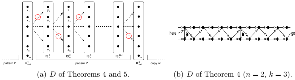
Figure 3: Digraph D described in Theorems 4 and 5.
