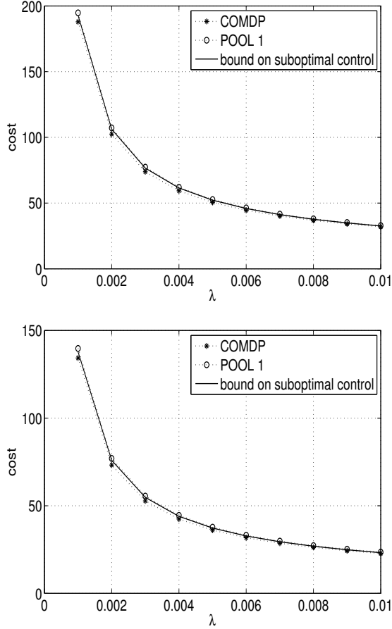
Fig. 3. Cost as a function of \lambda . The first set of plots is for the number of nodes N+1 = 51 and \eta = 2 while the second set of plots is for N+1 = 101 and \eta = 1 .
