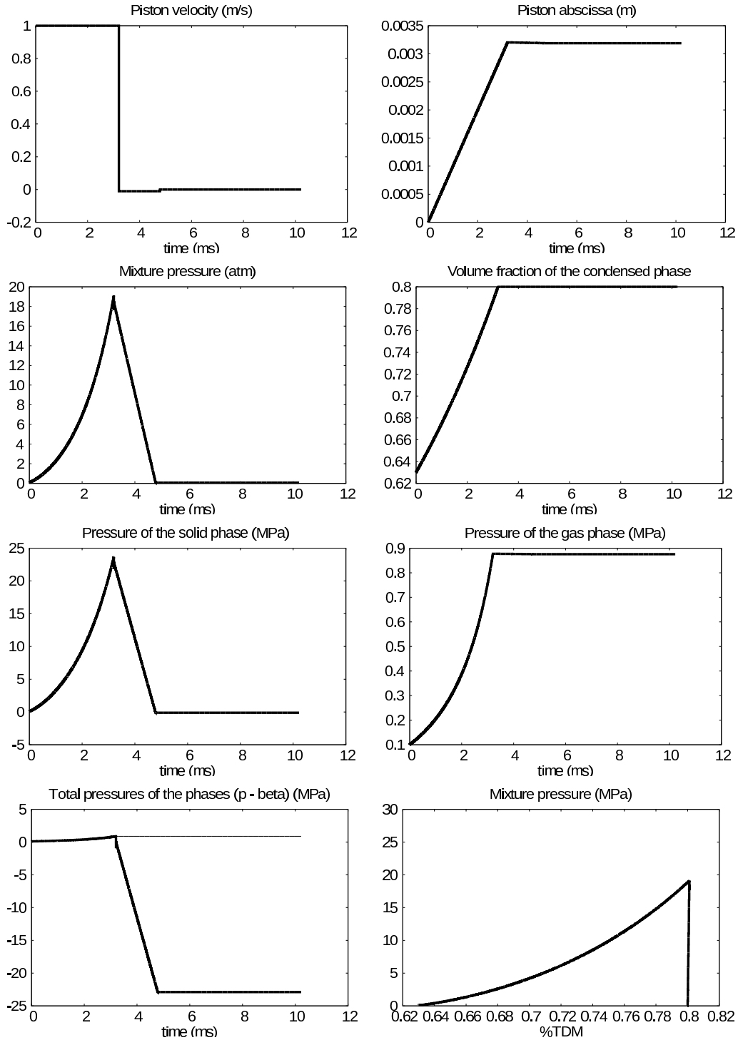
FIG. 6.34 Time evolution of the main flow variables for a loading–unloading cycle with HMX powder sample. The maximum value of the solid volume fraction set to 80 %, is reached at time t = 3 ms, and remains unchanged during the unloading stage. The hysteresis cycle is shown on the last right bottom graph.
