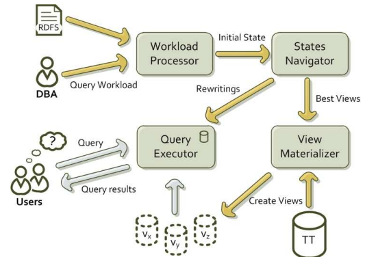
Figure 1: RDFViewS architecture.
