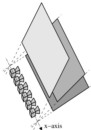
Figure 4. Epipolar planes.
