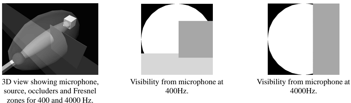
Figure 6: Using graphic hardware for “sound visibility” calculations.
