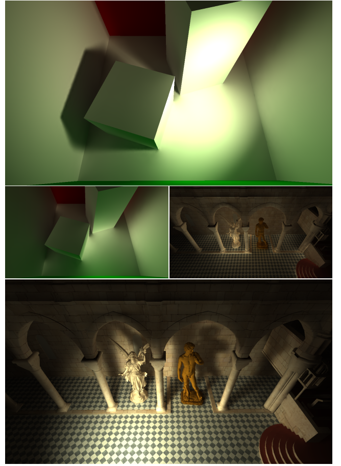
Figure 5: Radiosity images from two test scenes. Top: Cornell box final image. Bottom: Sibenik final image. Middle: the corresponding indirect-only images.
