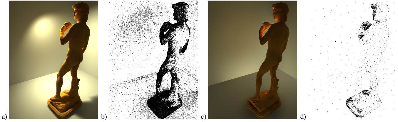
Figure 4: Michelangelo’s David. a) A meshless radiosity rendering of the statue. Note the complete absence of spurious discontinuities in the solution. c) The indirect component of the lighting. b) and d) The corresponding sparsity visualizations. The black points indicate non-zero coefficients, i.e., only their basis functions were touched during the radiosity simulation.
