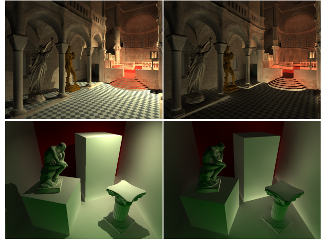
Figure 8: Screenshots from indirect diffuse PRT. Top: final and indirect-only images from Sibenik. Bottom: final and indirect-only images from Thinker. Per-pixel direct lighting was rendered using shadow maps.
