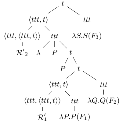
Fig. 10. Semantic derived trees for (1d) with the interpretation R_2(R_1(F_1, F_2), F_3)
