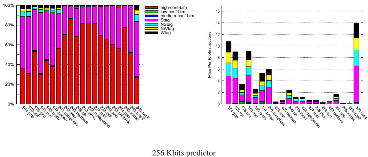
Figure 3: Distribution of predictions (left) and distributions of mispredictions (right) for the CBP-2 traces.
